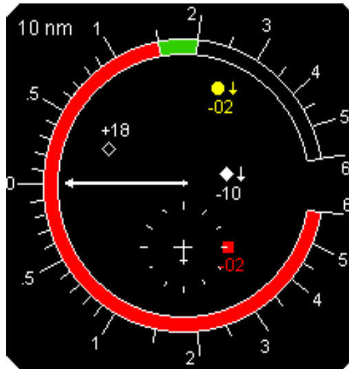
Typical TCAS II Display Figure 8
